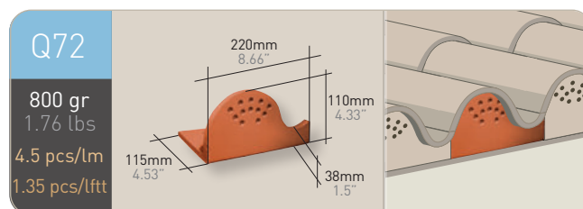
Bird stopper
